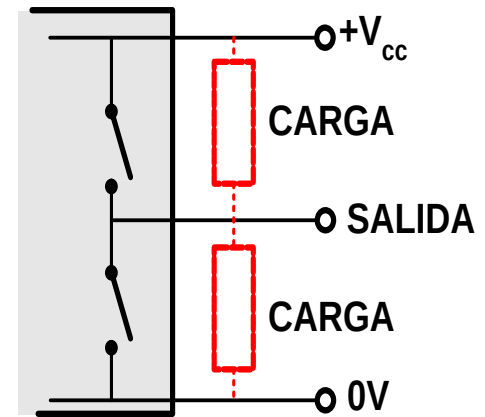
NPN-PNP
