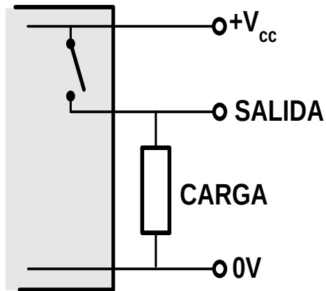
PNP
